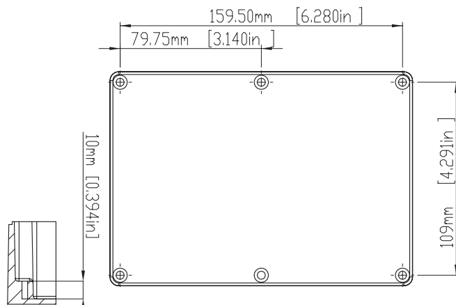
SECTION C-C
